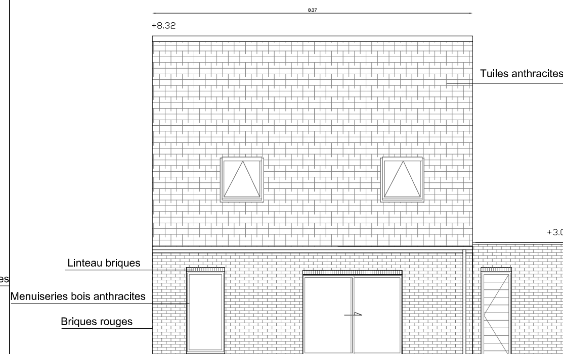
FACADE ARRIERE
